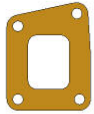
12191-1 CHRYSLER TURBO HOUSING INTAKE FLANGE
