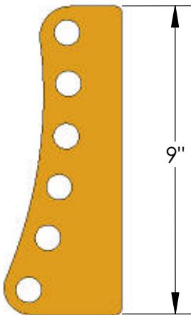
TRAILING ARM BRACKET-6 HOLE 12267-1 (1/2" HOLES) 12267-2 (5/8" HOLES) 12267-3 (3/4" HOLES)
