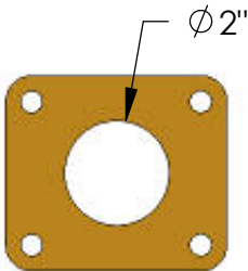
12196 TURBO T-4 FLANGE w/2.00" ROUND HOLE
