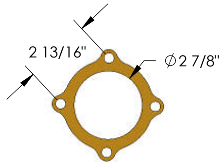
12197 SWITZER TURBO FLANGE
