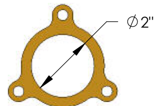
12200-1 2.000" ID 12200-2 1.625" ID T3 DISCHARGE FLANGE 2.00" ROUND 3 BOLT
