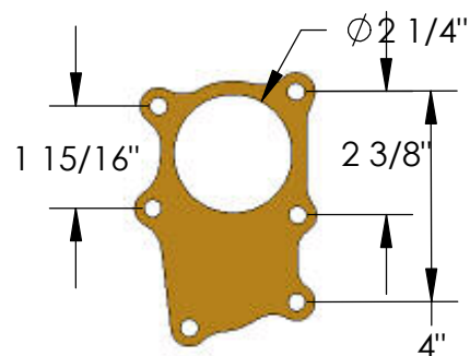
12203 NISSAN VG - 30
