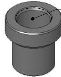
MD06-0007R OR MD06-0007L 2.0"OD X 1-1/4"-12 WELD IN ADAPTER FOR 2.0" X .250 WALL TUBE
