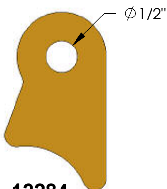
12284 3/16" MATERIAL
