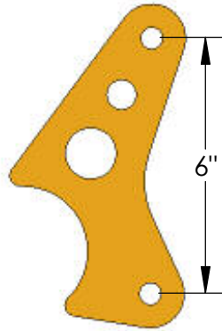
12268-1 (1/2" HOLES) 12268-2 (5/8" HOLES) 12268-3 (3/4" HOLES)
